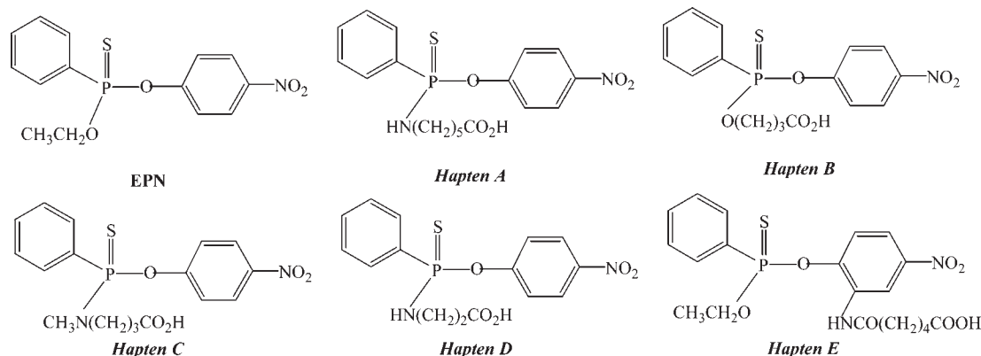
Figure 1. Structures of haptens for EPN.
